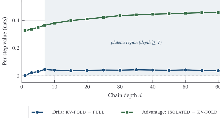
Figure 3: Drift saturates; advantage persists. Per-step drift (blue) and recurrence advantage (green) versus chain depth on Qwen2.5-7B-Instruct ( T = 16,384 , C = 256 ). Drift saturates at \sim 0.04 nats by depth 7 and remains flat through depth 63, while recurrence advantage stays positive throughout.
