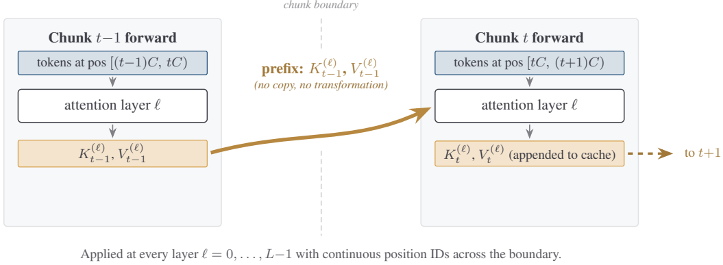
Figure 2: KV-Fold . Queries in chunk t attend to the KV cache from earlier chunks (amber) as a prefix; chunk t 's KV states are then appended and carried forward. No compression or additional parameters are introduced.
