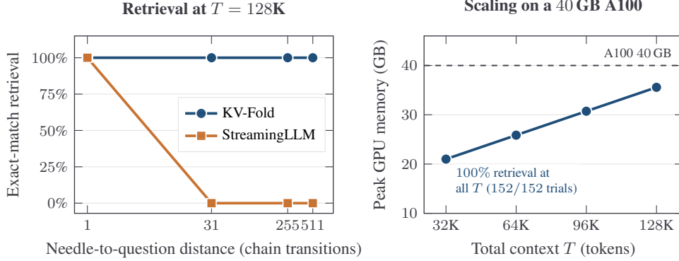
Figure 1: Headline result. Left: on Llama-3.1-8B at T = 128\text{K} , KV-Fold holds 100% exact-match retrieval at every tested distance through chain depth 511, while StreamingLLM falls to 0% once the needle exits its 1024-token cache. Right: peak GPU memory grows linearly at 0.13 KB per token; the chain at T = 128\text{K} , depth 511 completes in 171 s.
